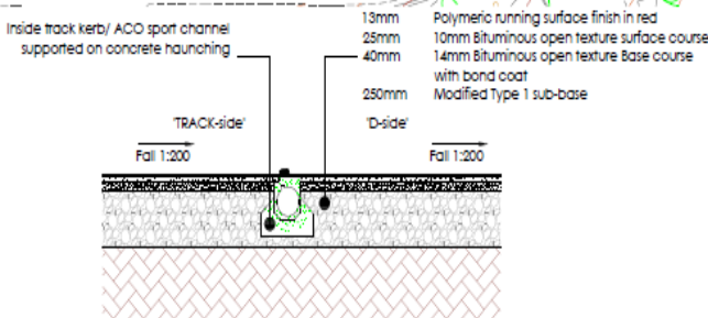
AA TYPICAL NEW POLYMERIC 'D' AREA SCALE: 1:20
